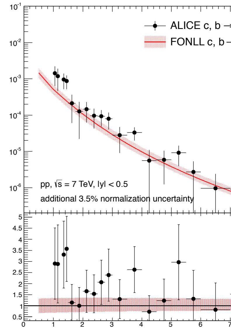
TPC+TOF (sec 11,12,13,14)
