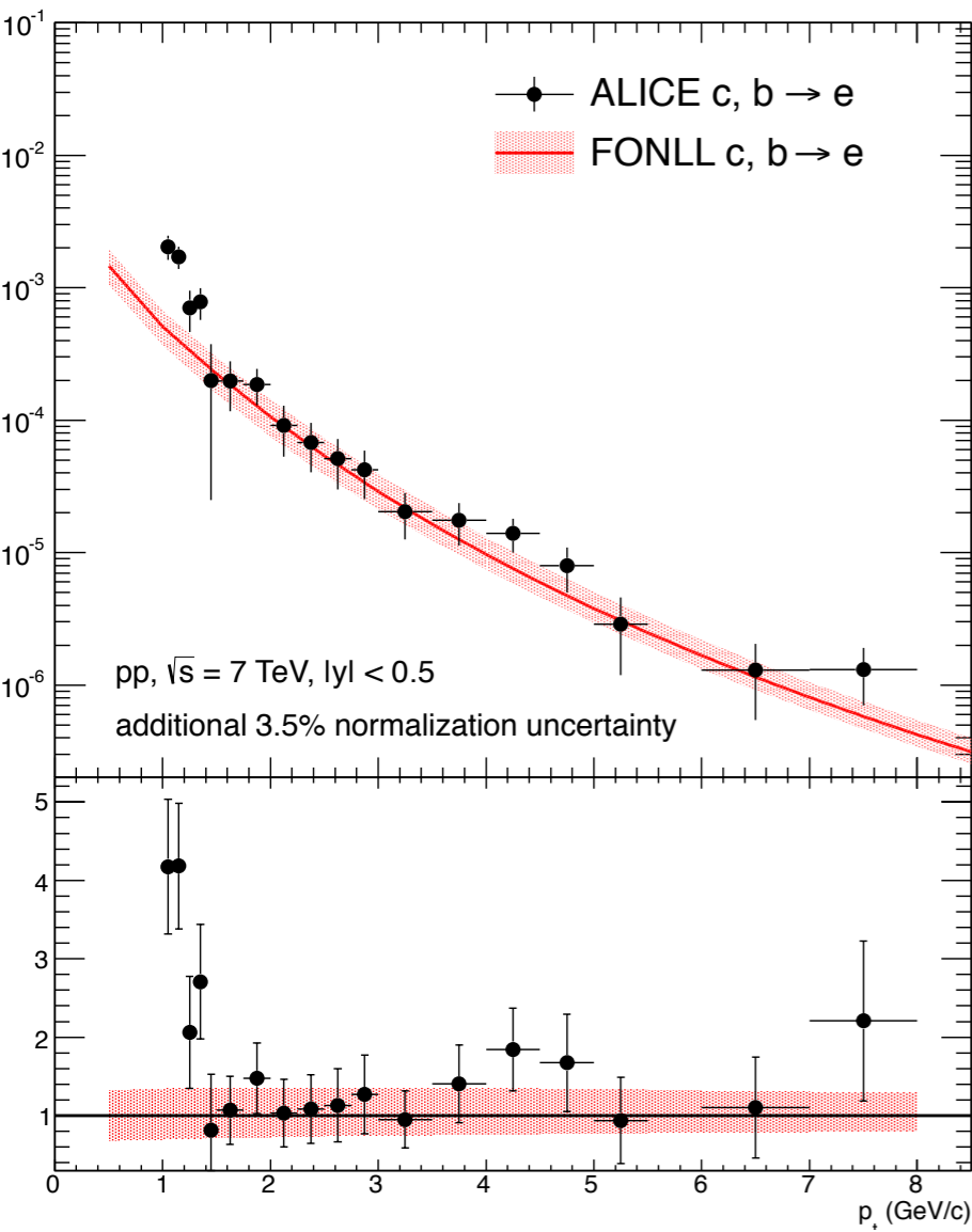
TPC+TOF (sec 7,8,9,10)
