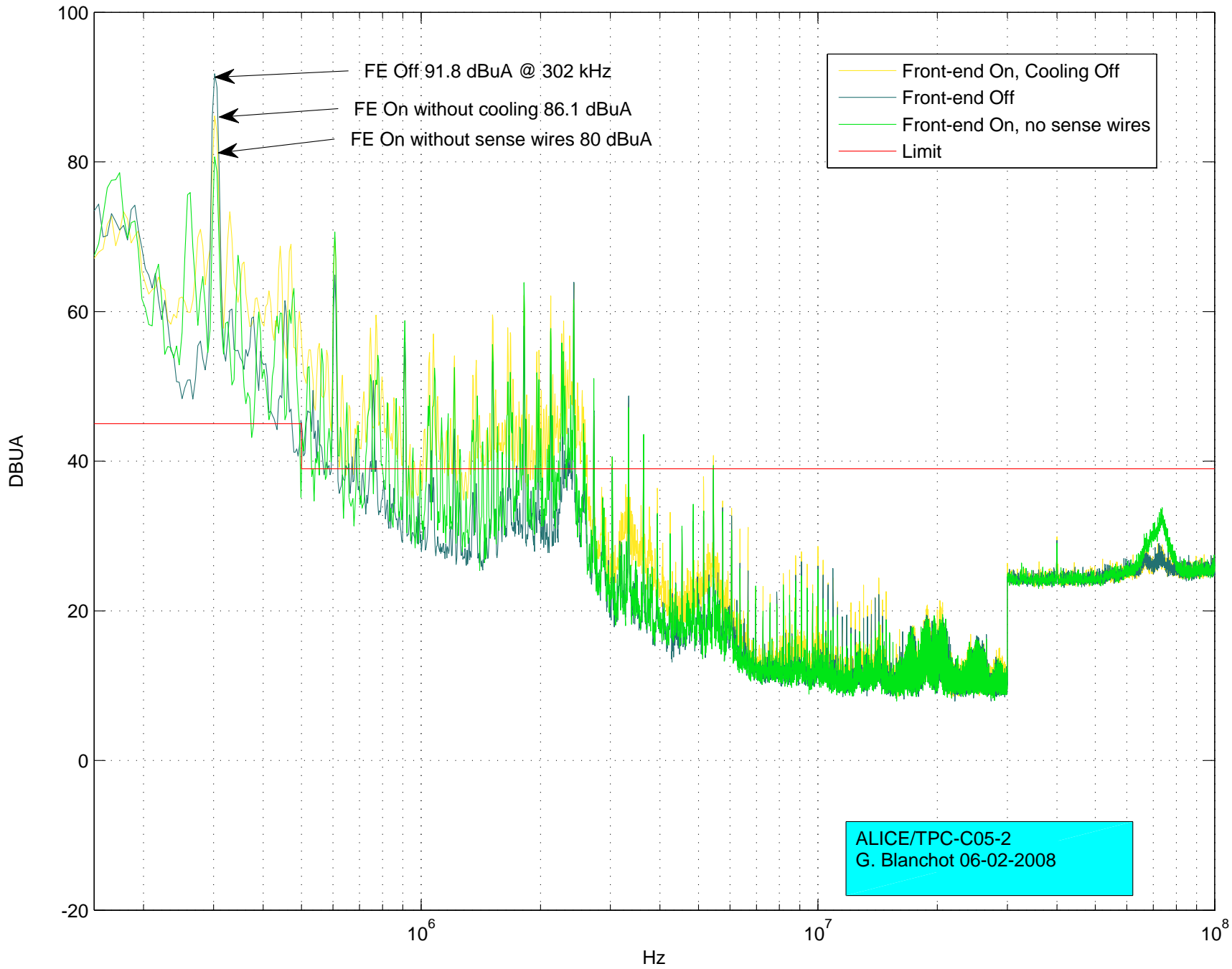
Alice TPC-C05-2 PL512 3.5VDIG 150ADC - Sense wires disconnected on trace 3
