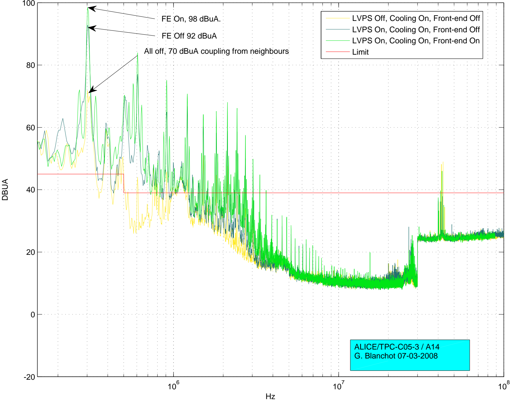
PL512 close to front-end using short cables, powering TPC-A14 (3.5VDIG 130A)
