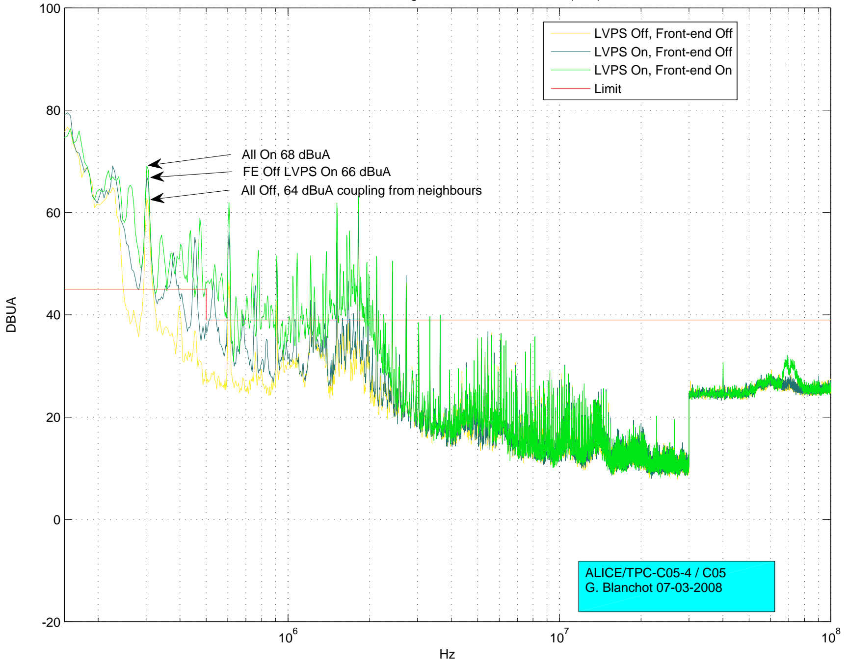
PL512 on scaffolding with ferrites on LV cables (C05)
